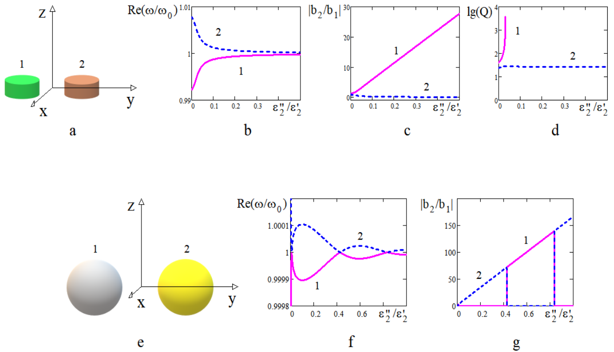
Fig. 1. Different cylindrical DR with main oscillations H_{101} (a) ( \epsilon_1''/\epsilon_1' = -0,01 ; \epsilon_{1r}' = \epsilon_{2r}' = 36 ; \Delta_1 = \Delta_2 = 0,4 ; f_0 = 10\text{GHz} ; \Delta x = \Delta z = 0 ; \Delta y = 10\text{mm} ). Different spherical DR with a whispering gallery mode H_{26,26,1} (e) ( \epsilon_{1r}' = \epsilon_{2r}' = 2,4 ; \Delta x = \Delta z = 0 ; k_0 \Delta y = 40 ). The coupling frequencies (b, f); amplitude ratio (c, g) quality factor of coupled oscillations (d) as functions of the complex dielectric constant tangent function of the second DR (a) ( \epsilon_1''/\epsilon_1' = -0,01 ).
